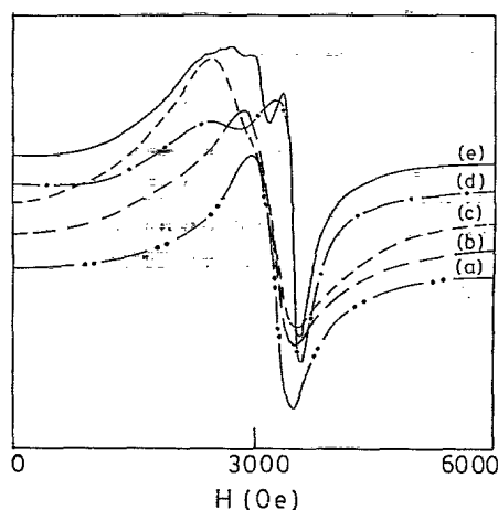
FIG. 6. Room-temperature ESR spectra of bismuth cuprate glasses recorded at a microwave frequency 9.44 GHz. (a) 27.15 mol % CuO (gain = 2.5 × 10 3 ), (b) 35.35 mol % CuO (gain = 4.0 × 10 3 ), (c) 45.70 mol % CuO (gain = 8.0 × 10 3 ), (d) 55.62 mol % CuO (gain = 5.0 × 10 3 ), and (e) 67.60 mol % CuO (gain = 6.3 × 10 3 ).
