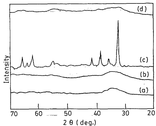
FIG. 1. X-ray diffractograms of several samples: (a) 27.15 mol % CuO, (b) 45.70 mol % CuO, (c) 45.70 mol % CuO heat treated at 500°C for 20 h, and (d) 67.60 mol % CuO.
