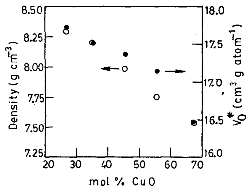
FIG. 3. Density (○) and oxygen molar volume (●) as a function of CuO content in the bismuth cuprate glass compositions.
