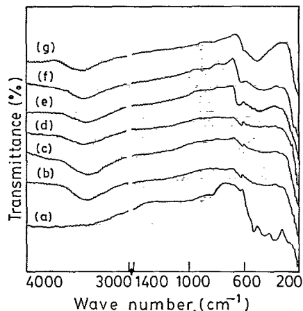
FIG. 5. Room-temperature infrared spectra of several samples: (a) crystalline Bi 2 O 3 , (b) 27.15 mol % CuO, (c) 35.35 mol % CuO, (d) 45.70 mol % CuO, (e) 55.62 mol % CuO, (f) 67.60 mol % CuO, and (g) crystalline CuO.
