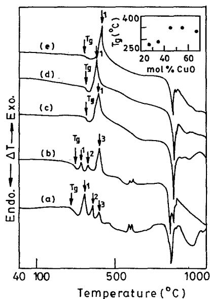
FIG. 4. Differential thermal analysis curves of several samples: (a) 27.15 mol % CuO, (b) 35.35 mol % CuO, (c) 45.70 mol % CuO, (d) 55.62 mol % CuO, and (e) 67.60 mol % CuO. ↓ indicated by T g is the glass transition temperature and ↓1, ↓2, etc. indicate crystallization temperatures. Inset shows glass transition temperature (T g ) as a function of CuO content.
